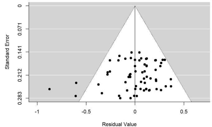
Fig. 1. Funnel plot of Fisher's z-transformed correlations between repetitive negative thinking and cognitive control.
